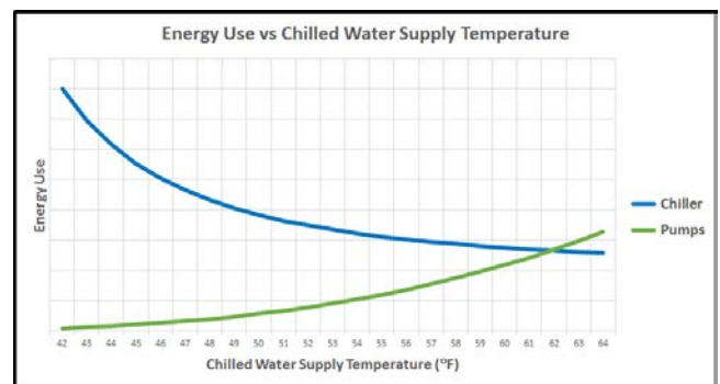
Figure 3: Simple Chiller and Pump Performance
