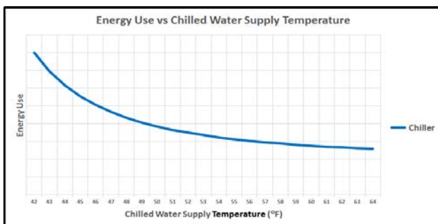
Figure 2: Simple Chiller Performance
