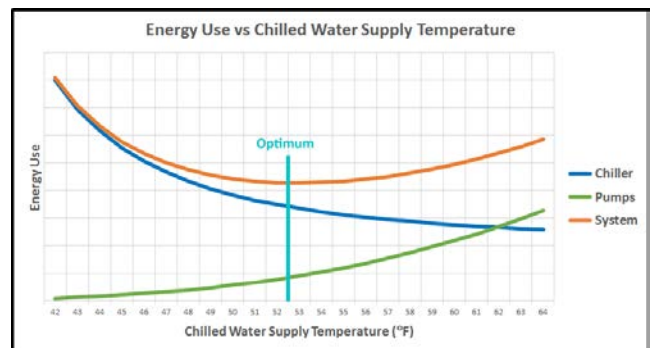
Figure 1: Total Chilled Water Supply System Energy
