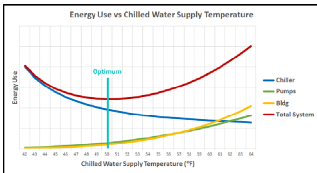
Figure 4: Chilled Water Energy Use including building load
